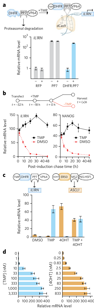
Figure 1 | Multidimensional 'chemical' control of endogenous transcript levels. (a) Top, small-molecule-mediated transcription induction via a destabilized domain-fused transcription activation domain (DHFR.PP7.VP64), dSpCas9, and an sgRNA. Bottom, HEK293T cells transfected with dSpCas9 and an RFP control, PP7.VP64, or TMP-regulated DHFR.PP7.VP64 targeted to IL1RN were treated with 10 \mu M TMP for 18 h before qPCR analysis. (b) Rapid turn-off of transcription. Cells were transfected and treated with 100 nM TMP to upregulate endogenous IL1RN (additional biological replicates are shown in Supplementary Fig. 3 ) or NANOG . After 18 h of TMP treatment, cells were provided with fresh media containing or lacking TMP before harvesting and analysis by qPCR. (c) Independent, small-molecule-mediated control of transcript expression for two genes in cells expressing dSpCas9 and two orthogonal destabilized domain-regulated transcription activation domains. DHFR.PP7.VP64 was targeted to IL1RN , and ER50.MS2.p65.HSF1 was targeted to ASCL1 . Transfected cells were treated as indicated (TMP, 100 nM; 4OHT, 10 nM) for 18 h before qPCR analysis. (d) Highly dose-responsive endogenous gene upregulation in cells transfected with dSpCas9, appropriate sgRNAs, and either DHFR.PP7.VP64 (left) or ER50.MS2.p65.HSF1 (right) targeted to IL1RN or ASCL1 , respectively. Transfected cells were treated with increasing concentrations of TMP or 4OHT for 18 h before qPCR analysis. Error bars represent \pm s.e.m. from biological replicates ( n = 3 ; a,c) or \pm s.d. across technical replicates ( n = 4 ; b,d).
